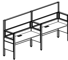
Two Persons Workstation (with glass) M60-2PP-1206 W1200*D600*H1650 M60-2PP-1506 W1500*D600*H1650 M60-2PP-1606 W1600*D600*H1650
