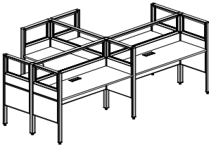
Four Persons Workstation (with glass) M60-4PN-1612 W1600/600*D1200/600*H1200 (L shape desk) W1200*600*H1200 (rectangular desk) M60-4PN-1616 W1600/600*D1600/600*H1200 (L shape desk) W1600*600*H1200 (rectangular desk)
