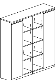
Cabinet M06-2WD-16165 W1600*D450*H1650
