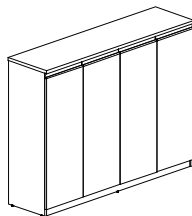
Cabinet M06-4WD-1612 W1600*D450*H1200
