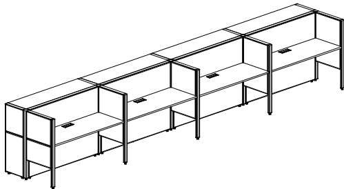
Four Persons Workstation (with cabinets) M60-4PO-1606 W1600*D600*H1200
