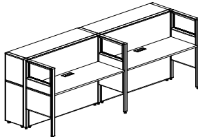
Two Persons Workstation (with cabinets) M60-2PL-1606 W1600*D600*H1200
