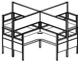
Four Persons Workstation (with glass) M60-4PR-1515 W1500/600*D1500/600*H1650 M60-4PR-1616 W1600/600*D1600/600*H1650
