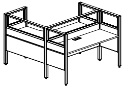
Two Persons Workstation (with glass) M60-2PJ-1612 W1600/600*D1200/600*H1200 (L shape desk) W1200*600*H1200 (rectangular desk) M60-2PJ-1616 W1600/600*D1600/600*H1200 (L shape desk) W1600*600*H1200 (rectangular desk)
