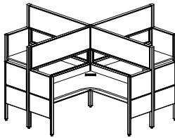
Four Persons Workstation (with glass) M60-4PQ-1515 W1500/600*D1500/600*H1650 M60-4PQ-1616 W1600/600*D1600/600*H1650
