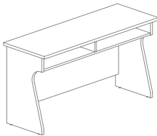
Training Desk (H600 modesty panel) RT1205 W1200×D500×H750 RT1405 W1200×D500×H750 RT1506 W1500×D600×H750 RT1606 W1200×D600×H750 RT1806 W1800×D600×H750
