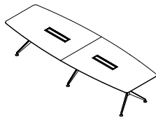
Model:MG-MM3012 3000W x 1200D x 750H Model:MG-MM3612 3600W x 1200D x 750H
