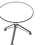
Model:MG-MR0909 900W x 900D x 750H
