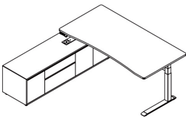
主桌带左边柜(不含指纹锁) Main desk with cabinet on left hand (without finger print lock) HAT-MCL-NLK-1818 W1800*D900 / W1800*D500 HAT-MCL-NLK-2018 W2000*D900 / W1800*D500
