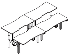
四工位 Four persons workstations HAT-WD3014 W3000*D1400 HAT-WD3614 W3600*D1400
