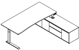
主桌带右边柜(不含指纹锁) Main desk with cabinet on right hand (without finger print lock) HAT-MCR-NLK-1818 W1800*D900 / W1800*D500 HAT-MCR-NLK-2018 W2000*D900 / W1800*D500
