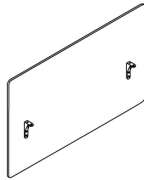
独立桌挂台屏风 Screen for single table HAT-SH1275 W1200*D12*H750 HAT-SH1575 W1500*D12*H750
